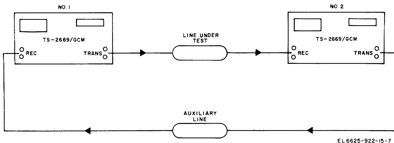
Figure 3-4. Connections for end-to-end with return reference.
