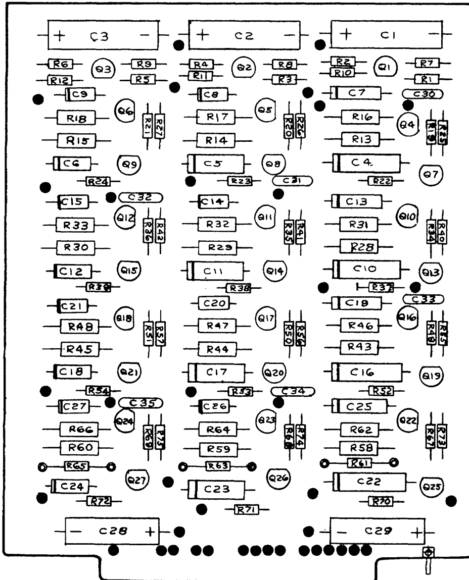
Figure 9-15. Lowpass active filter (A13), C-4699-2, location of components.
