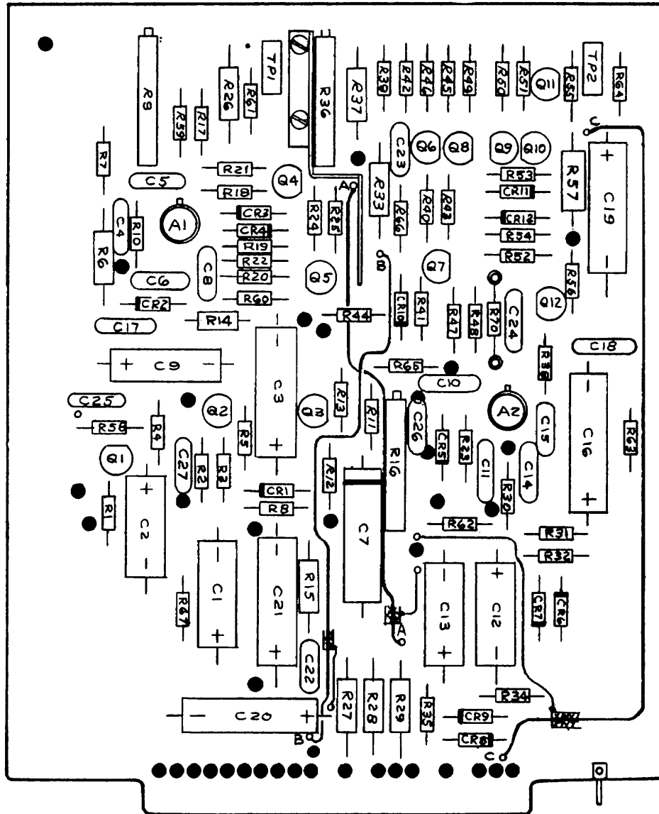
Figure 9-19. Output amplifier and meter amplifier (A12), C-4704, location of components.
