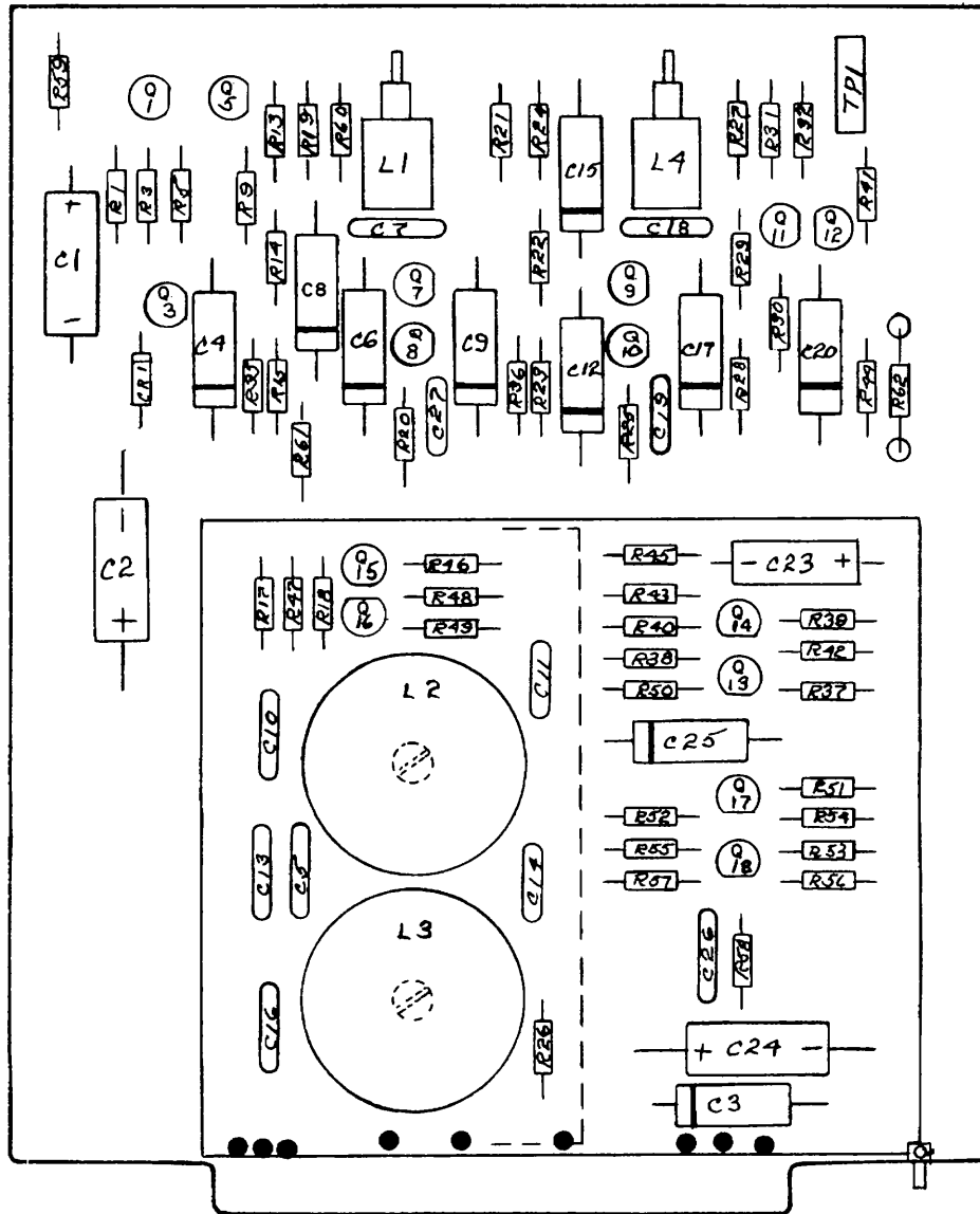
Figure 9-12. 200-kHz modulator mixer (A15), C-4706, location of components.
