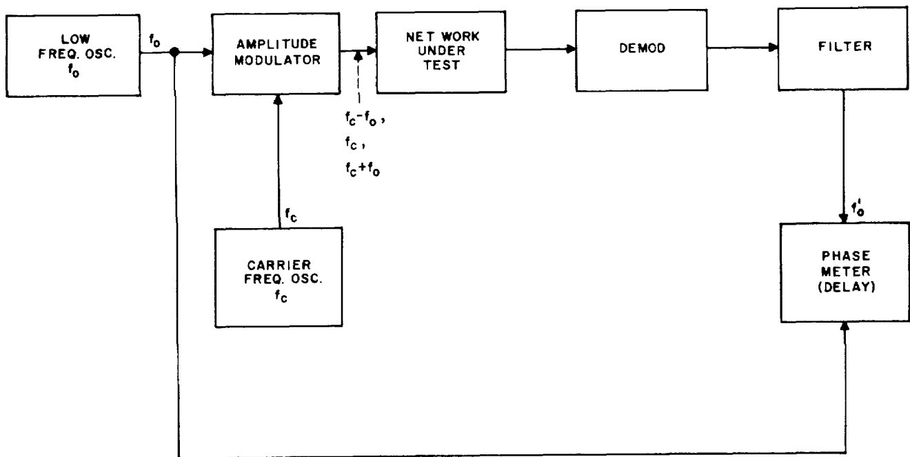
Figure 5-1. Time Delay.
