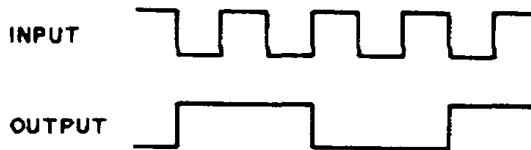
C. DUAL FLIP-FLOP, SN7473N, IN DIVIDE-BY-4 MODE
