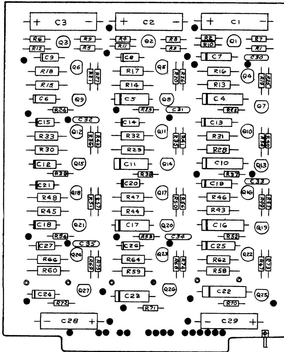
Figure 9-14. Low-pass active filters (A7), C-4699-1, location of components.
