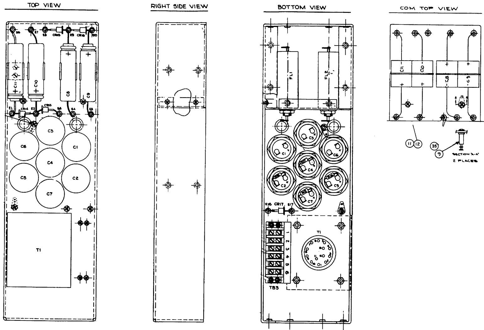
Figure 9-36(3). Assembly drawing (part 3 of 4).
