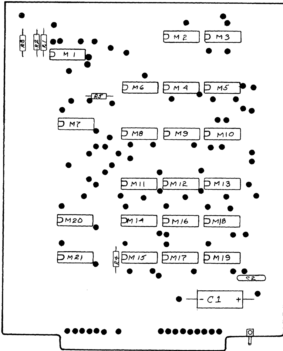
Figure 9-25. Countdown logic (A10), C-4702, location of components.
