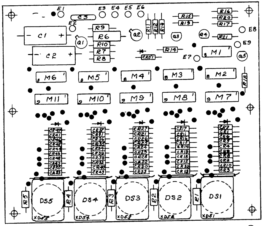
Figure 9-29(1). Frequency counter/display (A1), D-4637, location of components (part 1 of 2).
