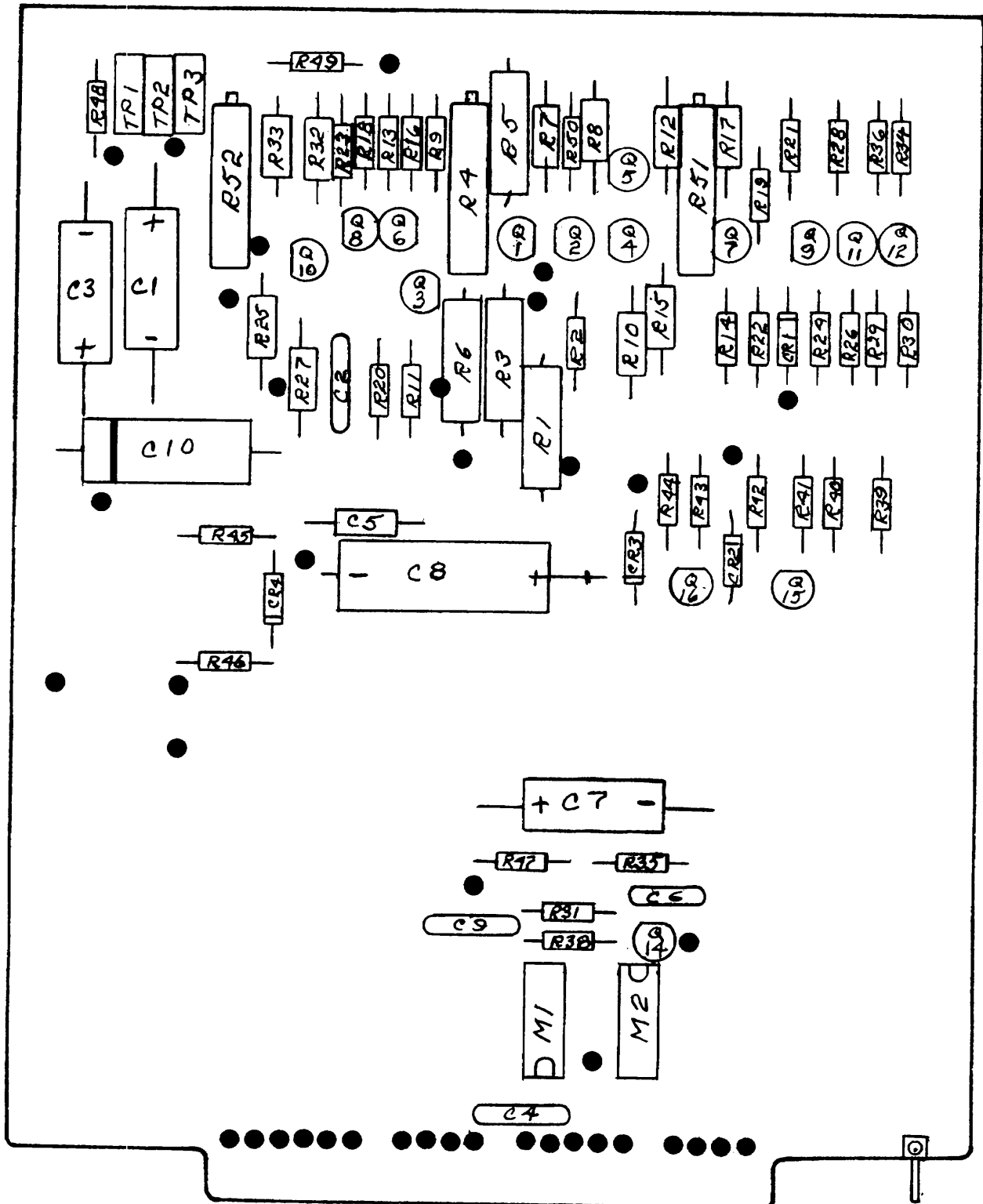
Figure 9-8. Sweep drive (A16), C-4707, location of components.
