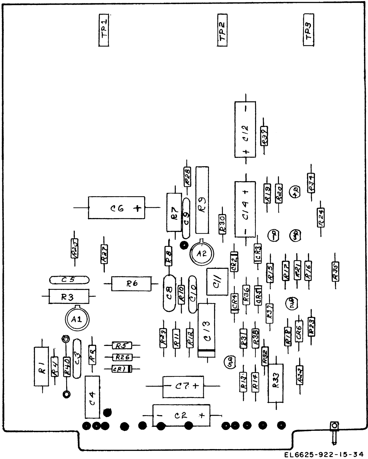
Figure 9-17. Input amplifier and demodulator (A6), C-4698, location of components.
