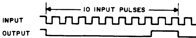
D. DECADE COUNTER, SN7490N, IN DIVIDE-BY-10 MODE
