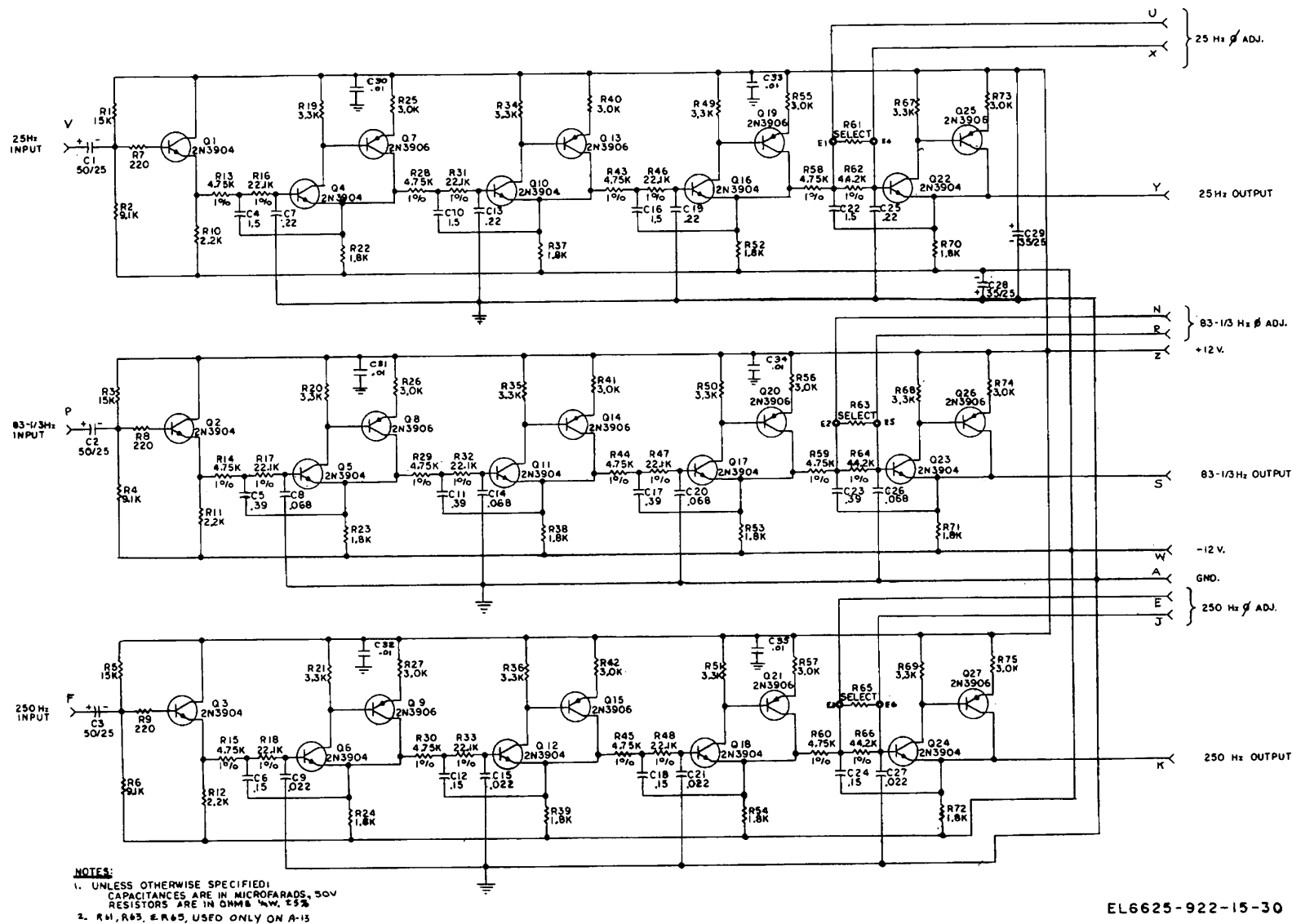
Figure 9-13. Low-pass active filters (A7, A13), C-4699-1, C-4699-2, schematic diagram.
