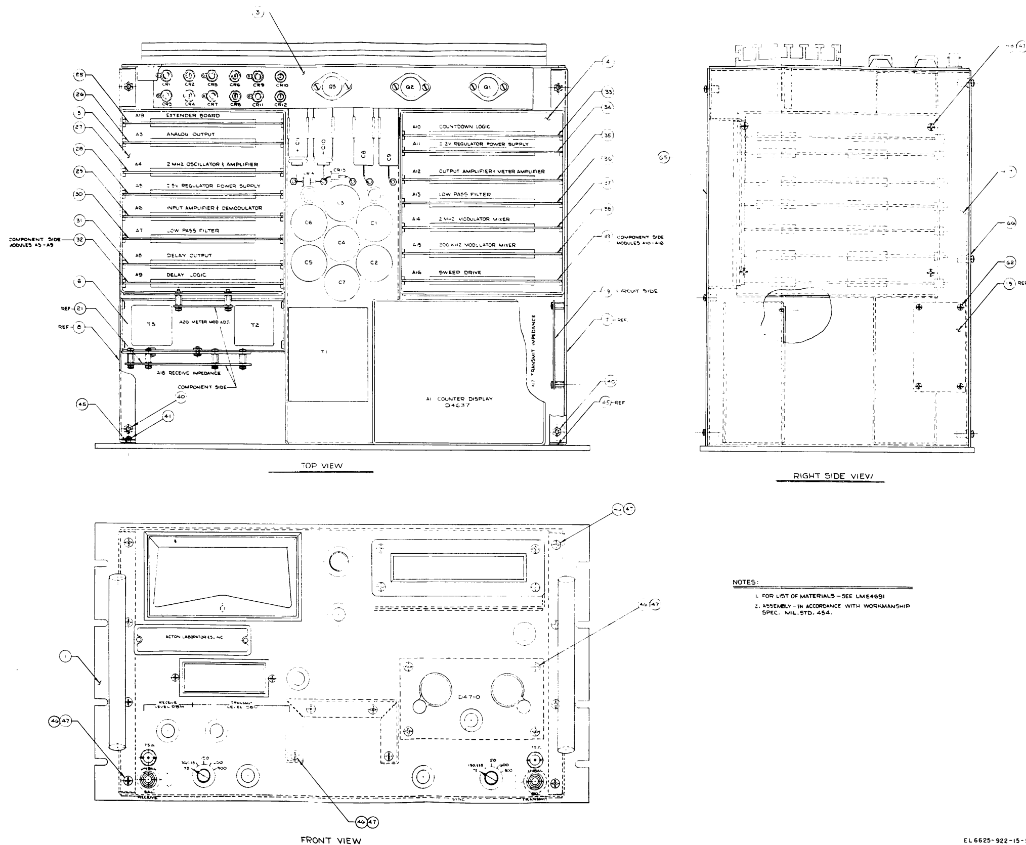
Figure 9-6(1). Assembly drawing (part 1 of 4).
