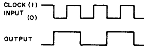
B. FLIP-FLOP IN DIVIDE-BY-2 MODE
