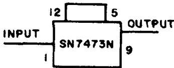
C. DUAL FLIP-FLOP, SN7473N, IN DIVIDE-BY-4 MODE
